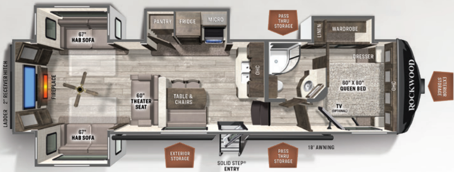
2898KS REAR LIVING ULTRA LITE U/VW: 9631 HITCH: 1583 AXLE: 7989 CCC: 1952 LENGTH: 36' 6" WIDTH: 8' HEIGHT: 13' 2" FRESH: 54 gal GRAY: 90 gal BLACK: 50 gal
