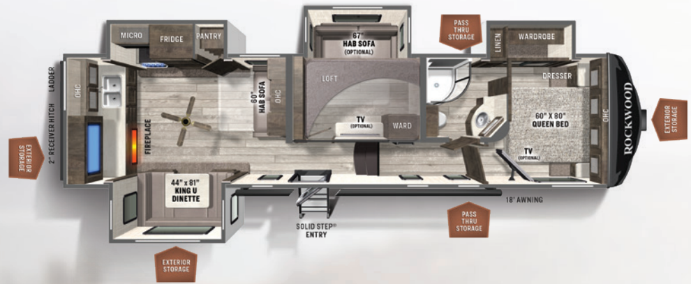
2896MB BUNKHOUSE ULTRA LITE U/VW: 9662 HITCH: 1588 AXLE: 8015 CCC: 1926 LENGTH: 36' 6" WIDTH: 8' HEIGHT: 13' 2" FRESH: 54 gal GRAY: 90 gal BLACK: 50 gal
