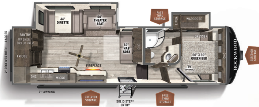
2881S REAR KITCHEN ULTRA LITE U/VW: 8758 HITCH: 1308 AXLE: 7391 CCC: 2550 LENGTH: 33' WIDTH: 8' HEIGHT: 13' 2" FRESH: 54 gal GRAY: 80 gal BLACK: 40 gal
