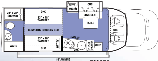
15' AWNING TS2370 (Ford EcoBoost 3.5L gas engine)
