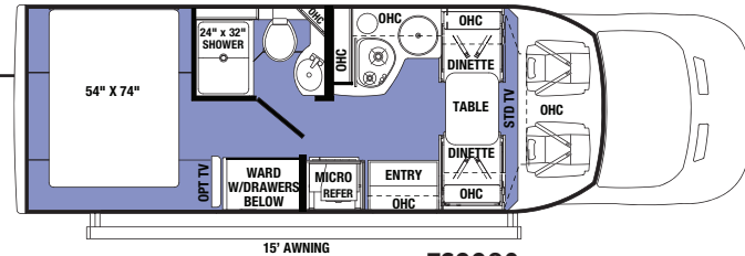
15' AWNING TS2380 (Ford EcoBoost 3.5L gas engine)
