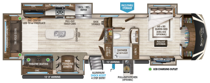
385GK UVW' HITCH' GVWR LENGTH' HEIGHT CAPACITY 385GK-R 13,336 2,724 16,800 40' 6" 13' 5" 93 106 53
