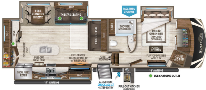
344GK UVW' HITCH' GVWR LENGTH' HEIGHT CAPACITY 344GK-R 12,600 2,500 16,800 36' 11" 13' 5" 93 100 50
