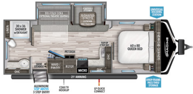
2600RB UVW 1 5,795 HITCH 1 594 LENGTH 2 29' 8" HEIGHT 11' 1" CAPACITY 52 82 45
