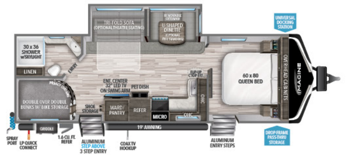
2800BH UVW 1 6,386 HITCH 1 604 LENGTH 2 32' 0" HEIGHT 11' 1" CAPACITY 52 82 45
