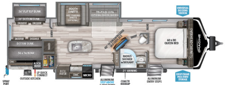
3250BH UVW 1 8,496 HITCH 1 844 LENGTH 2 36' 11" HEIGHT 11' 4" CAPACITY 52 90 45
