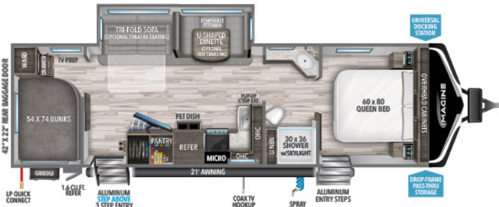
2910BH UVW 1 7,087 HITCH 1 720 LENGTH 2 33' 11" HEIGHT 11' CAPACITY 52 90 45
