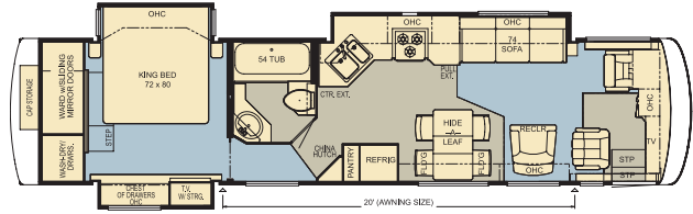
DSDP 3816 Options: K030, K124_3, K420_2, K541
