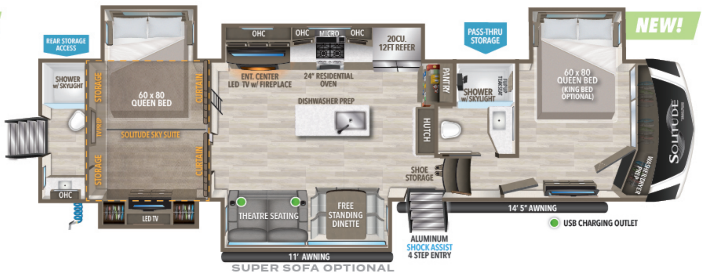
391DL UVW † 15,300 HITCH ‡ 3,050 GVWR 16,800 LENGTH † 43' 11" HEIGHT 13' 5" CAPACITY 81 106 106
