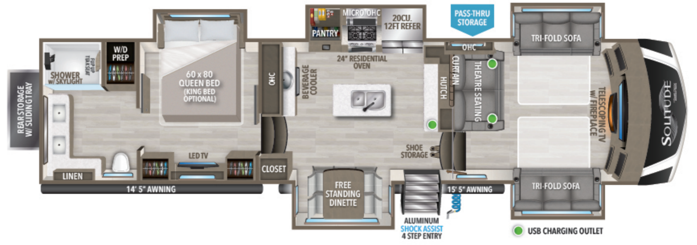
382WB UVW † 14,866 HITCH ‡ 3,052 GVWR 16,800 LENGTH † 41' 5" HEIGHT 13' 5" CAPACITY 81 106 53
