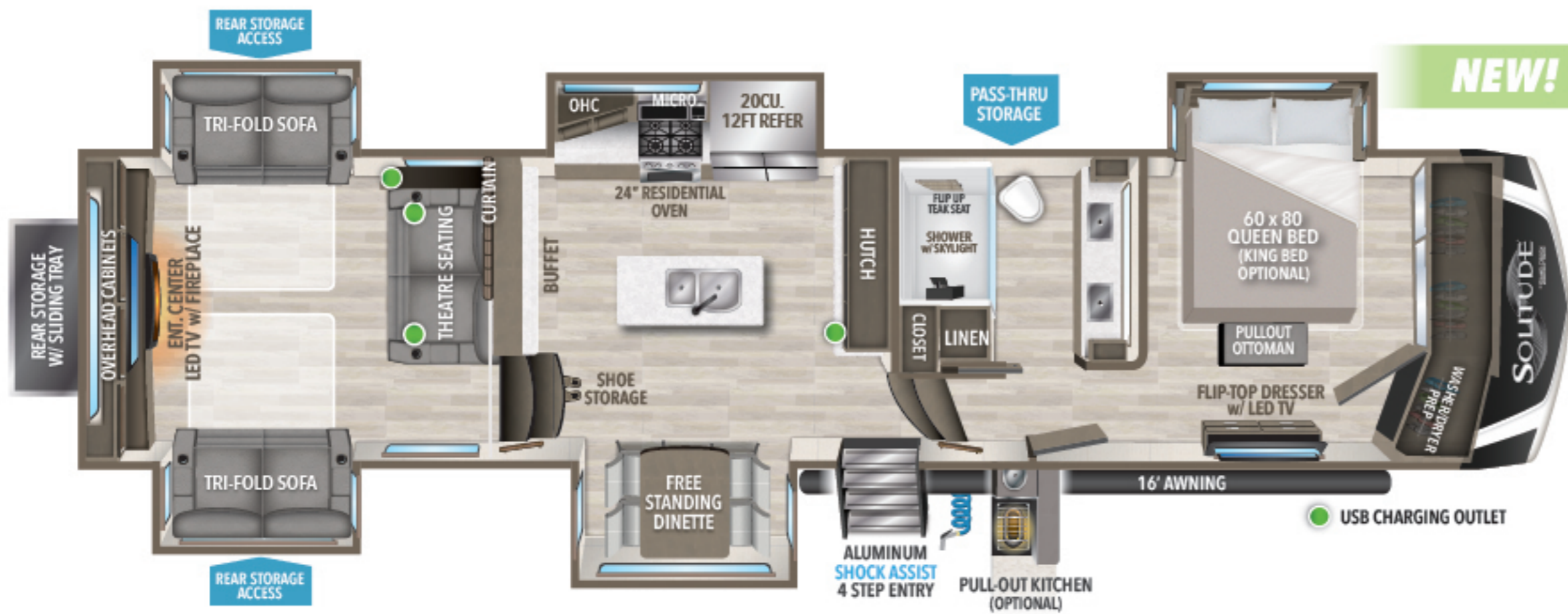
376RD UVW † TBD HITCH ‡ TBD GVWR 16,800 LENGTH † 42' 6" HEIGHT 13' 5" CAPACITY 81 106 53
